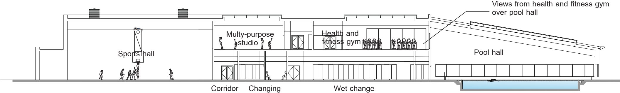
Typical cross Section
