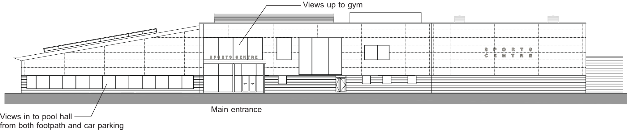
Front elevation (North)
