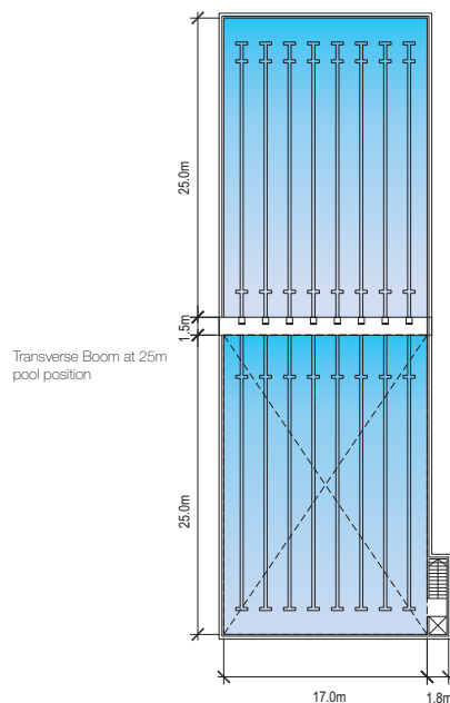
Configuration 2 - 25 m mode 25 m lane swimming / training 1.8 m deep in both halves or 1.8 m deep in one half and variable depth on other half
