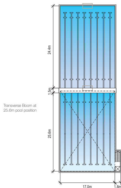
Configuration 4 - Women's water polo mode Women's water polo + 1 no. smaller pool - fixed depth
