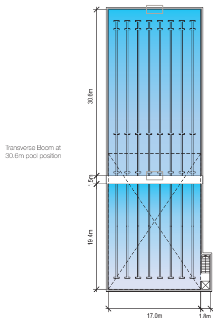
Configuration 3 - Men's water polo mode Men's water polo + 1 no. smaller pool - fixed depth
