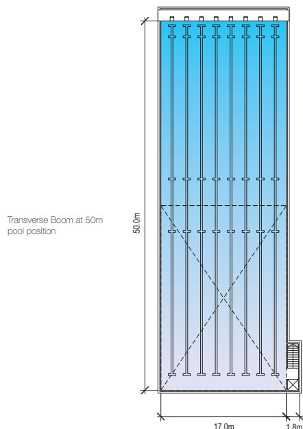
Configuration 1 - 50 m mode 50 m lane swimming / training 1.8 m deep
